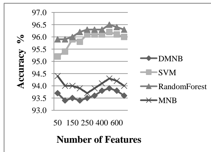
Figure. 4. The results for IG filter and dual-word terms
