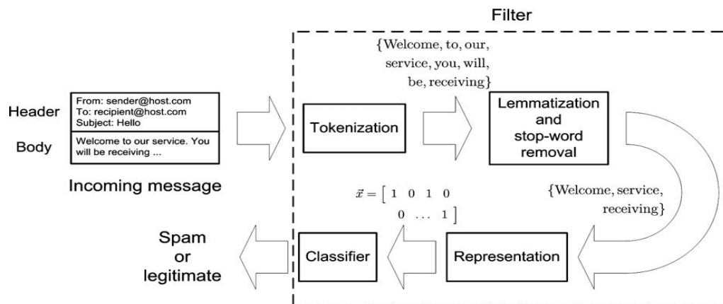
Figure 1. An illustration of some of the main steps involved in a spam filter
