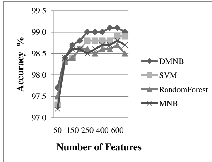
Figure. 3. The results for IG filter and uni-word terms
